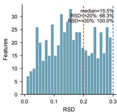
D Pooled-QC RSD distribution
