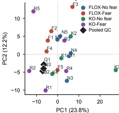
A PCA with pooled QC
