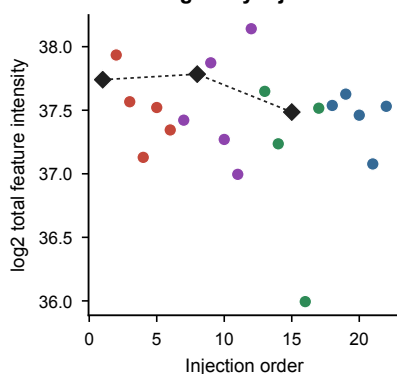
E Total signal by injection order
